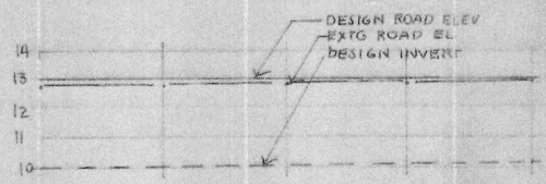
PROFILE ELEVATION
