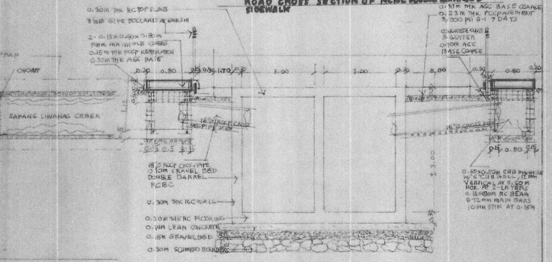
ROAD CROSS SECTION OF RCRC DOUBLE BARREL BOX CULVERT WITH MANHOLE
