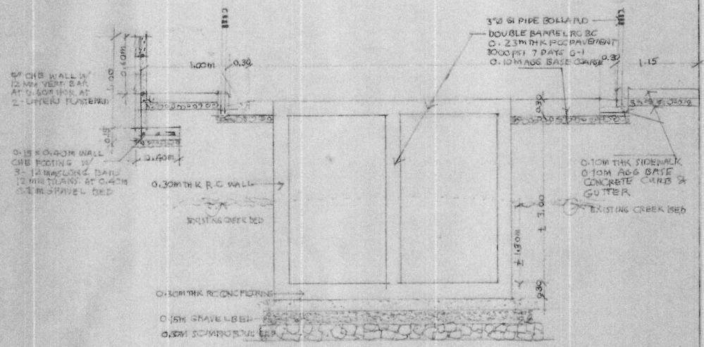
ROAD CROSS SECTION OF RCRC DOUBLE BARREL BOX CULVERT
