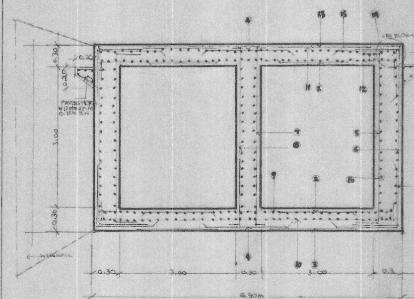
DETAIL OF REINFORCED DOUBLE BARREL RCBC (3.0m x 3.0m DOUBLE)
