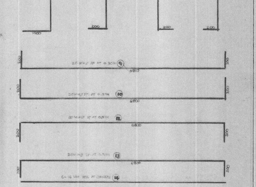
BAR BENDING DIAGRAM FOR DOUBLE BARREL RCBC
